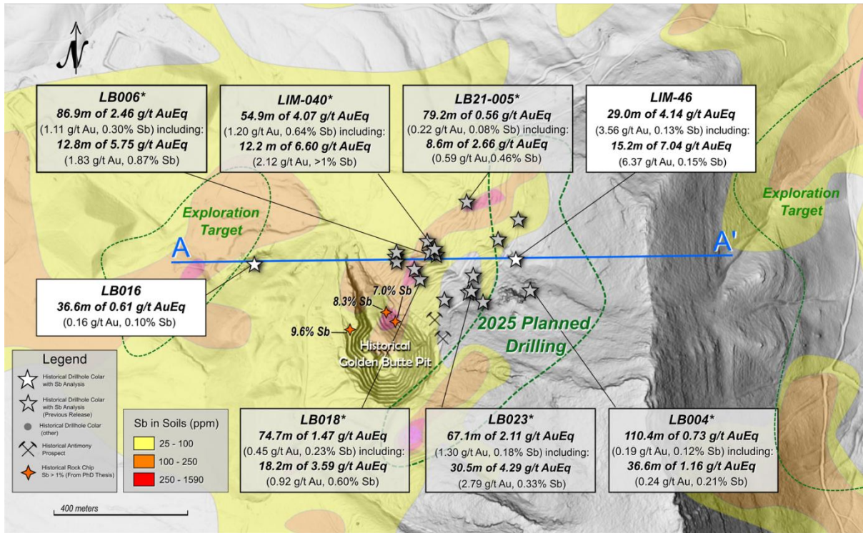
Figure 1 – Limousine Butte Gold-Antimony Project with selected gold-antimony drillhole results.
